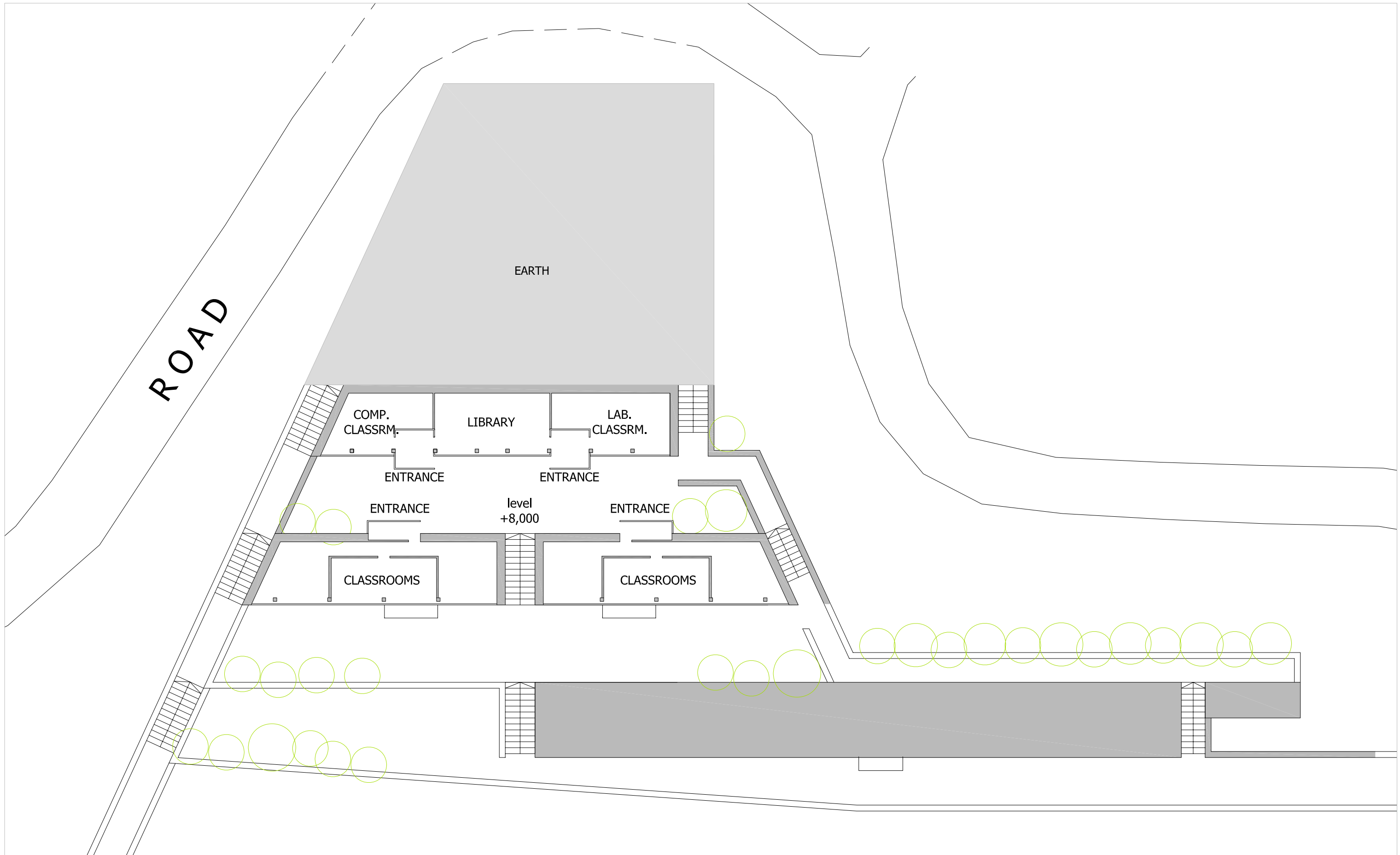
PROPOSED LAYOUT LEVEL +08.0
