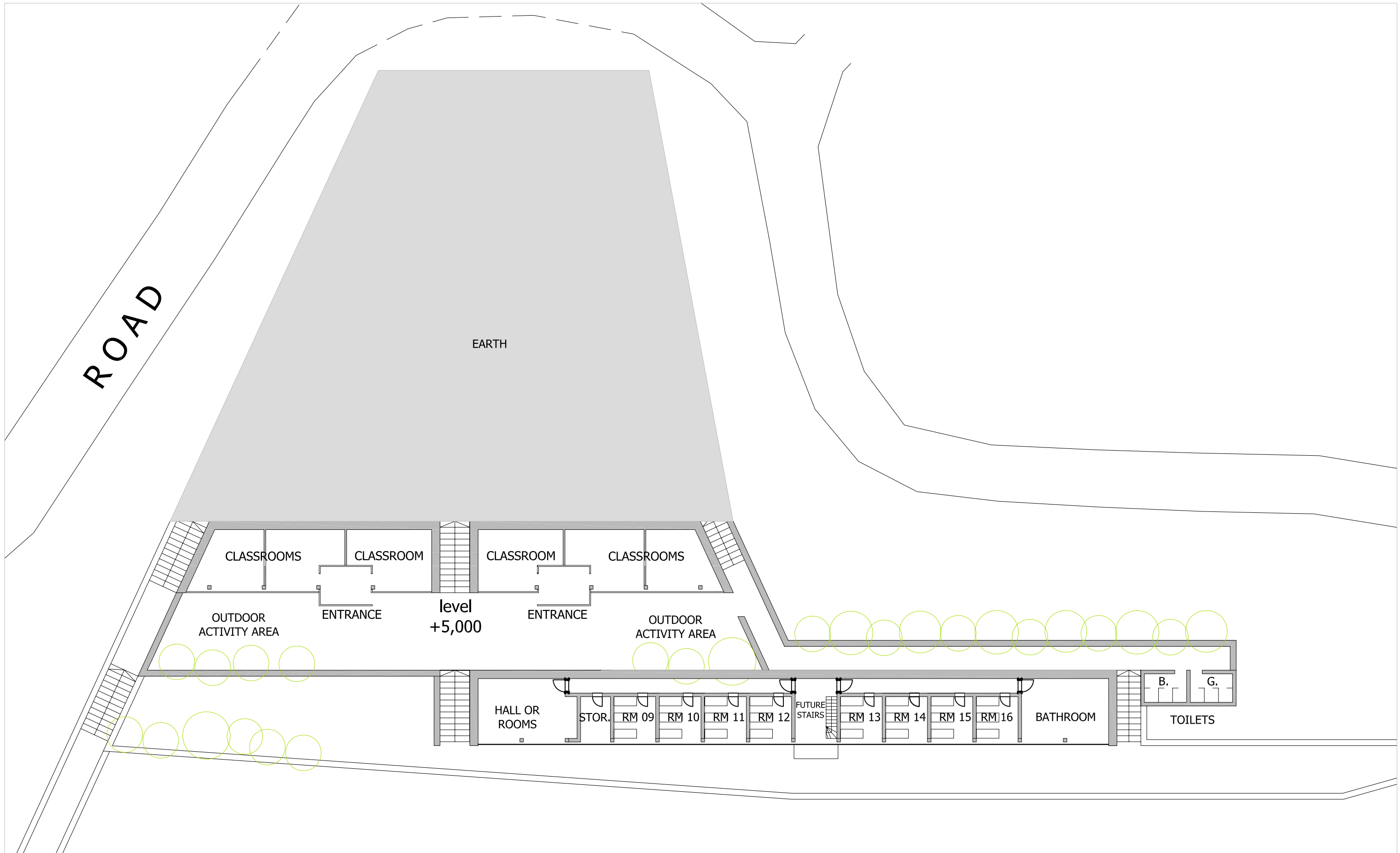
PROPOSED LAYOUT LEVEL +5.0
